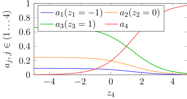
Figure 3.1.: Equation (78) for different fixed values of z_{1,2,3}^L and variable z_4^L . L index avoided for clarity.
